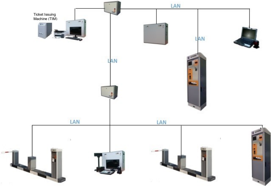
Logical Layout diagram for Central Database Engine (CDE)
